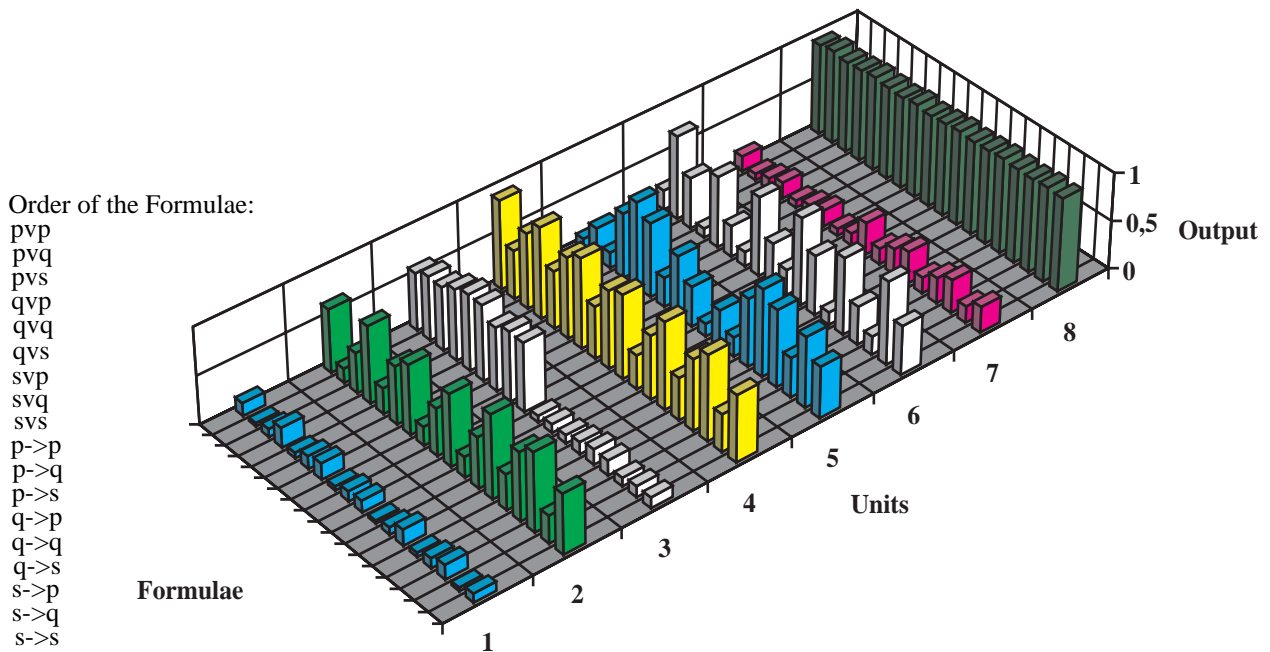
Figure 6: Hidden-layer representations
