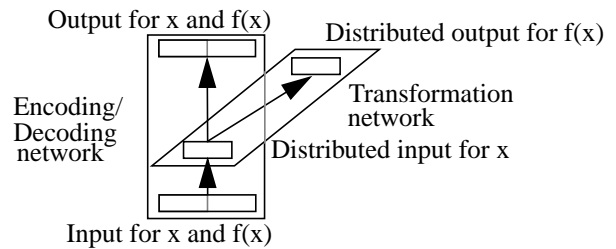
Figure 3: Our architecture
