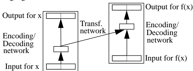
Figure 2: Chrisman's architecture
