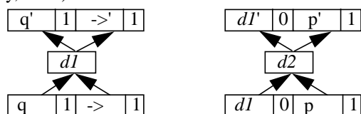
Figure 5: Automatic decoding
